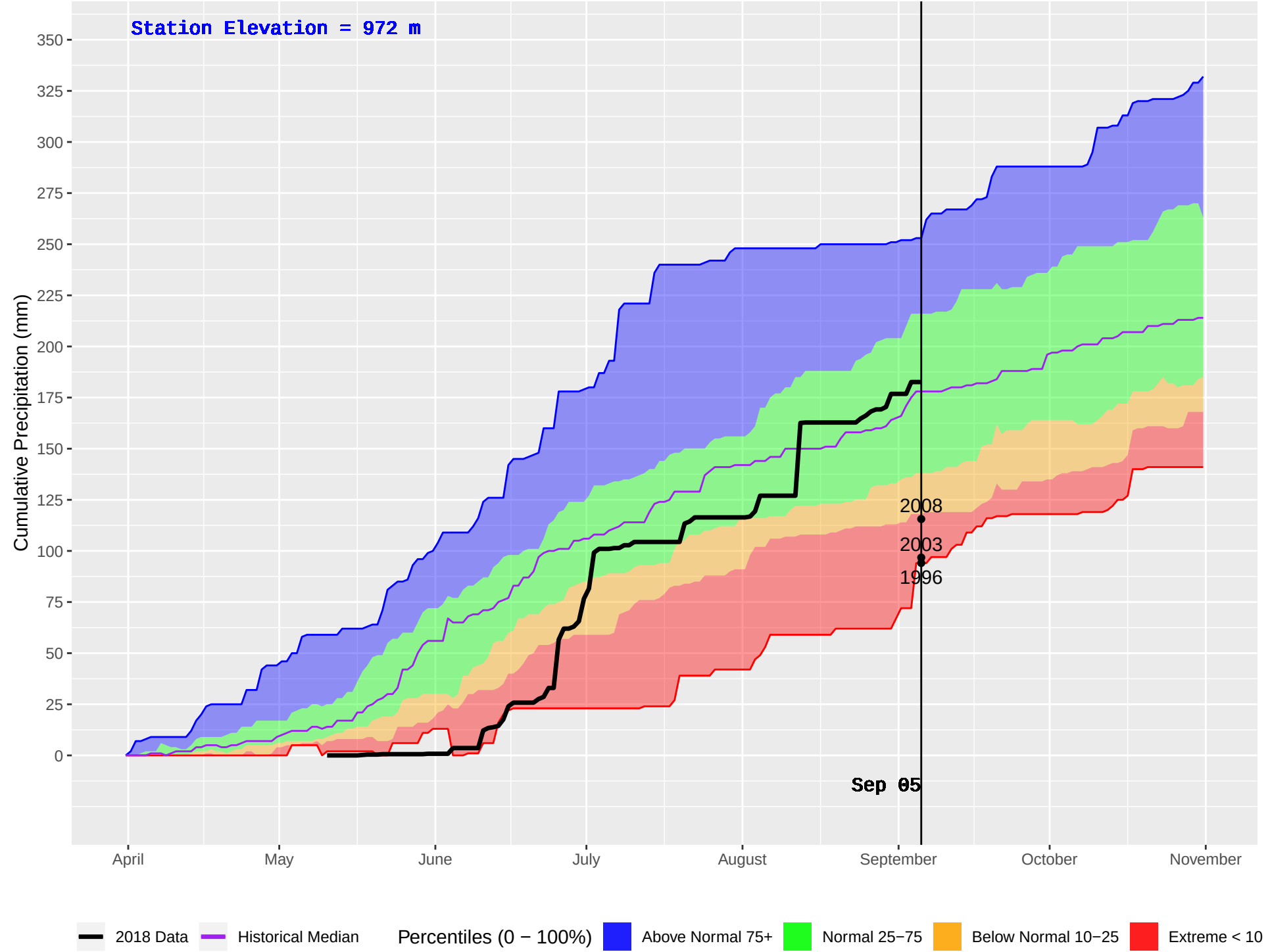
SPARKS LAKE (305) : Historical (1991–2016) and Current (2018) Daily Cumulative Precipitation
