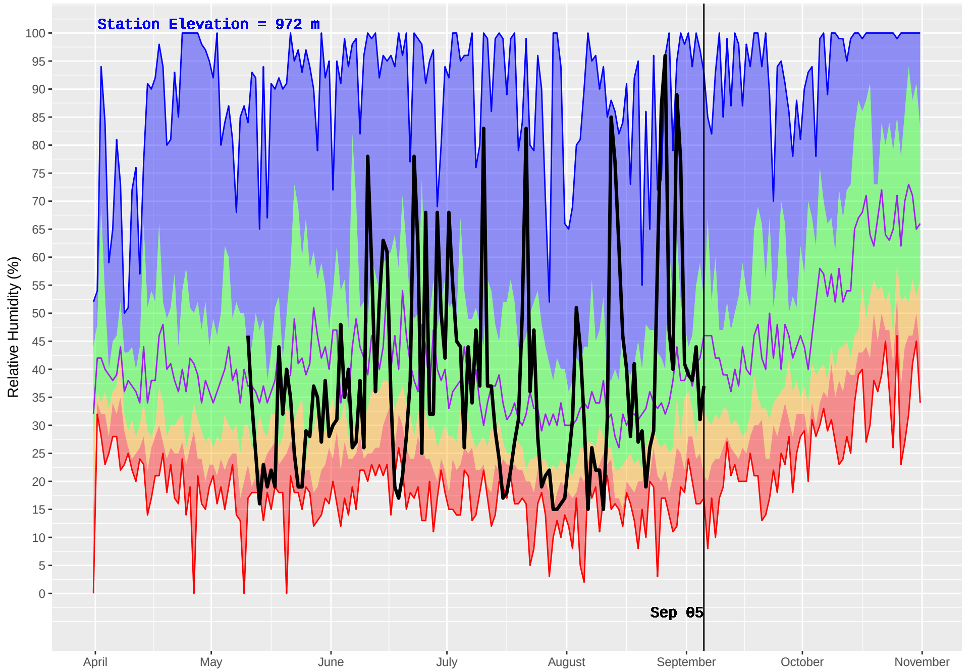
SPARKS LAKE (305) : Historical (1991–2016) and Current (2018) Daily Relative Humidity
