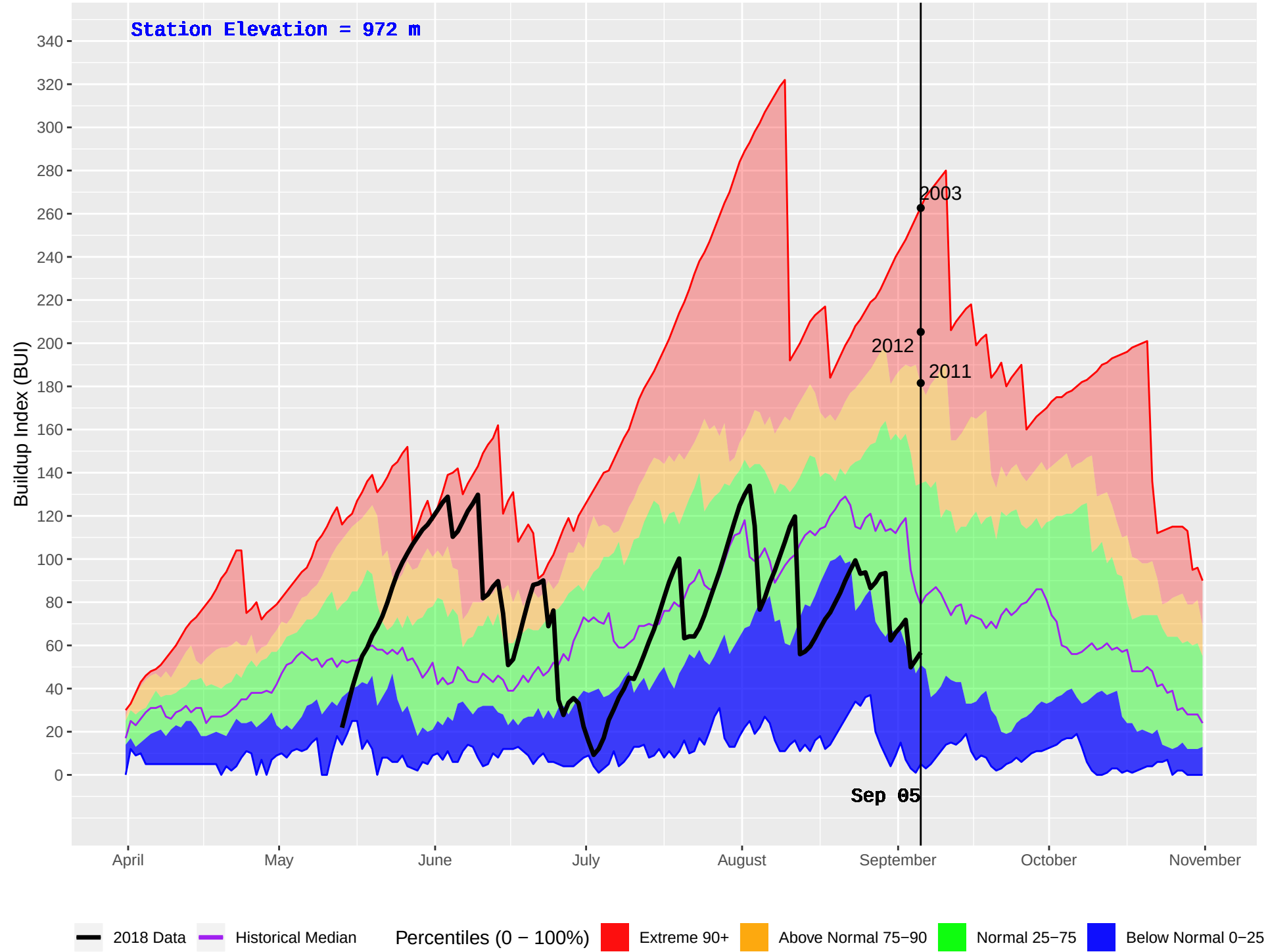
SPARKS LAKE (305) : Historical (1991–2016) and Current (2018) Daily Buildup Index (BUI)
