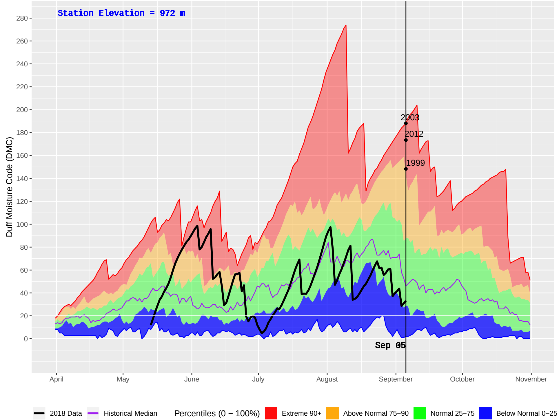
SPARKS LAKE (305) : Historical (1991–2016) and Current (2018) Daily Duff Moisture Code (DMC)
